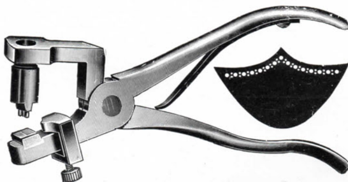
FANCY PUNCH PLYER for Toe Caps, &c., with adjustable guide.
