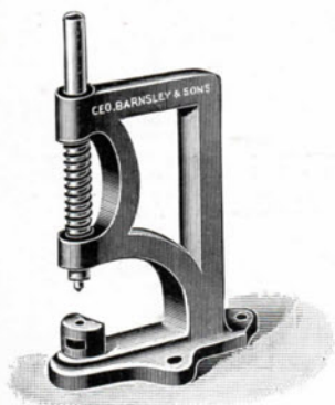
Code 4426. Pattern No. 3. SMALL SPRING HOOK EYELET MACHINE, to strike with hammer.
