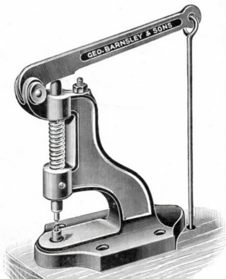
Code 4422. Pattern No. 1. FOOT POWER MACHINE with 0, 1, and 2 Punch and Eyelet Closing Bits.
